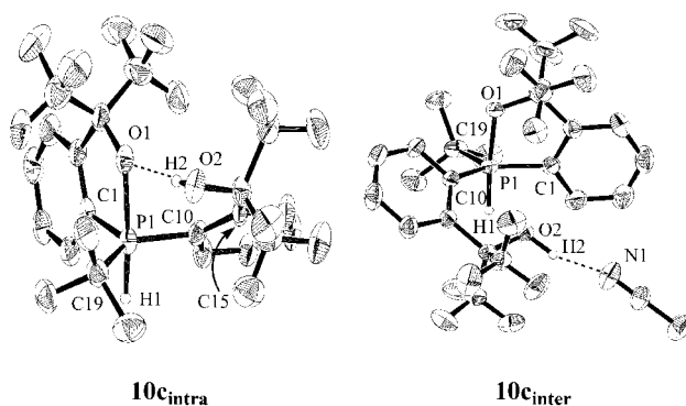
Figure 2. ORTEP drawings of 10c intra and 10c inter showing the thermal ellipsoids at the 30% probability level. All the hydrogen atoms other than P1–H1 and O2–H2 have been omitted for clarity. The broken lines denote hydrogen bonding.
